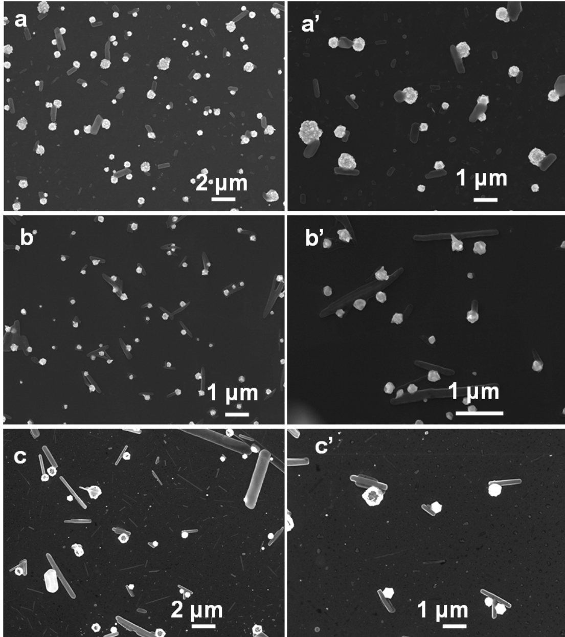
Figure 49. FESEM results of KCP rods induced from GNPs with various diameters in 0.3 M K_2[Pt(CN)_4] \cdot 3H_2O aqueous solutions with applied potential of 1.5 V and applied time of 1s. Figure (a'-c') are high magnification images for Figure (a-c).
