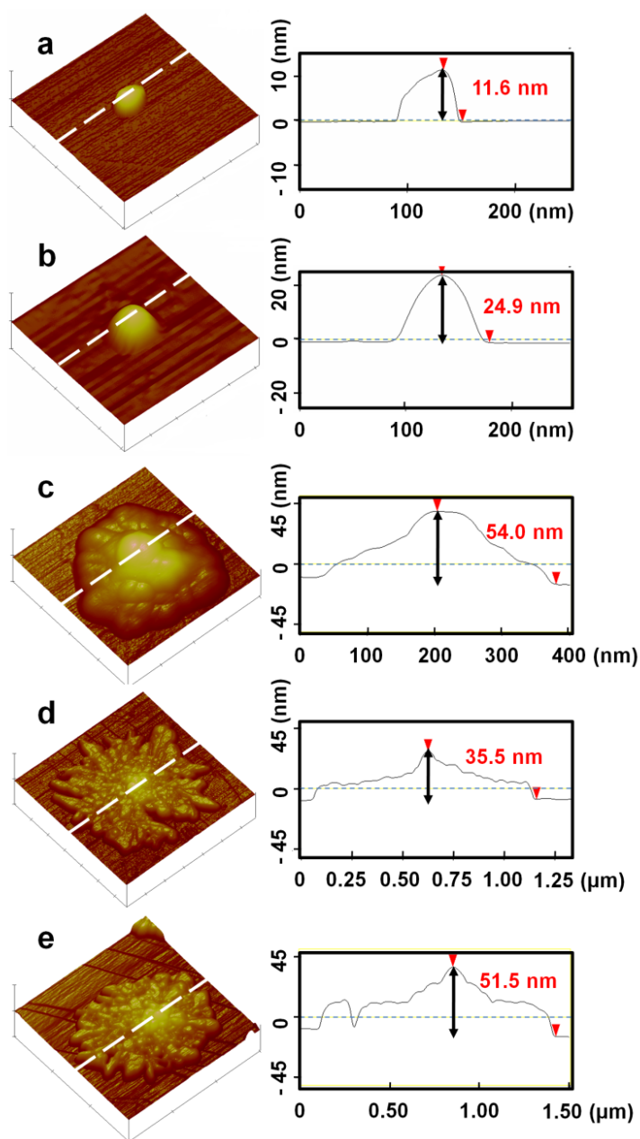
Figure 30. The 3D surface plot (left) and sectional height analysis (right) of AFM images of single GNP electrodeposition on freshly cleaved HOPG. GNP is electrodeposited from (a) 0.1 mM; (b) 0.5 mM; (c) 1 mM; (d) 5 mM; and (e) 10 mM \text{HAuCl}_4 at overpotential of -0.5 V for 10 ms. The sectional height analysis is measured along the dashed white line on their corresponding 3D surface plot image. Z range is 20 nm for (a), 30 nm for (b), 100 nm for (c-e).
