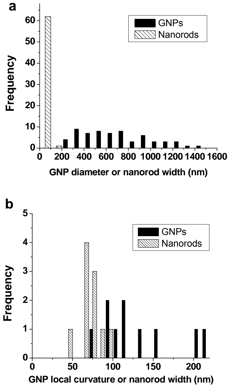
Figure 40. Size distribution for the diameter (a) and local curvature (b) of the dendritic GNPs and the width of their induced (TTF)Br 0.76 crystals.
